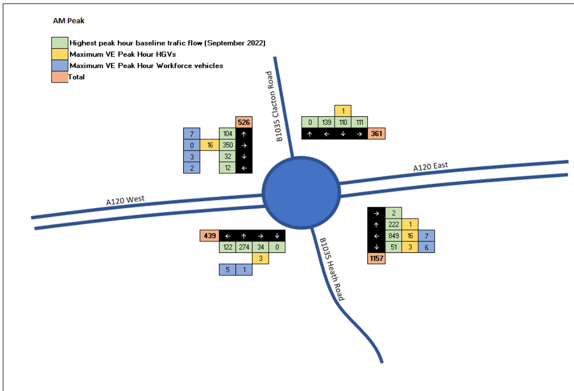
Figure 6-7: Forecast Maximum Morning Peak Hour VE Construction Vehicle Movements at the A120/ B1035 Roundabout
